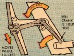
Fig. 2. Unless the steering wheel is allowed some play when you come to a hot stop, the bell crank goes into action—like we've shown in gray—and pivots the wheels to the left.
