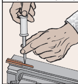
Swage loose locking spring
