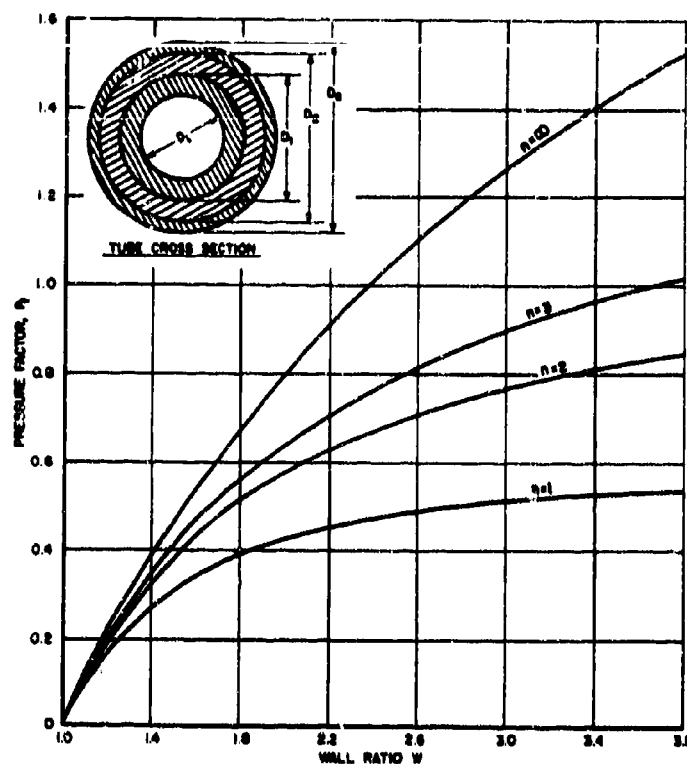
FIGURE 33. Wall Ratio-Pressure Factor Curves for Multilayer Tubes.
