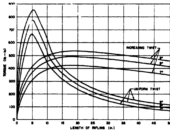
FIGURE 30. Effects on Rifling Torque by Varying Exit Angle.
