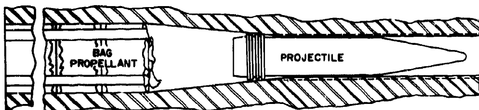
(d) ARTILLERY CHAMBER CONTAINING SEPARATELY LOADED ROUND
