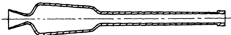
FIGURE 7. Recoilless Gun Tube.
