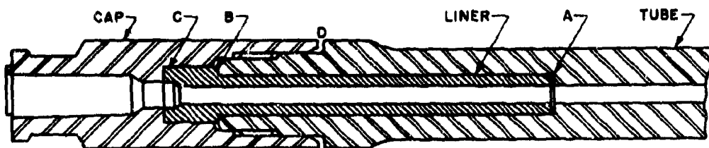
FIGURE 4. Quasi Two-Piece Tube.
