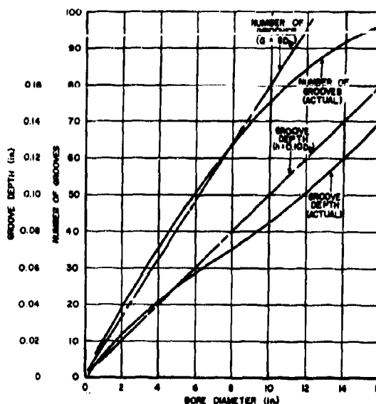
FIGURE 26. Groove-Bore Relations.
