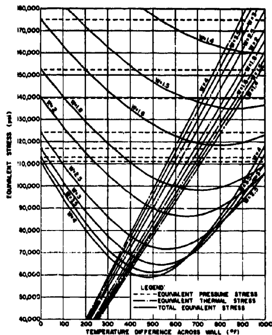
FIGURE 40. Equivalent Stress as a Function of Wall Thickness Ratio and Temperature Distance for an Internal Pressure of 80,000 psi.
