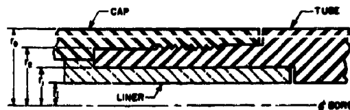
FIGURE 63. Schematic of Tube With Liner.
