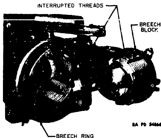
FIGURE 51. Interrupted Threads.
