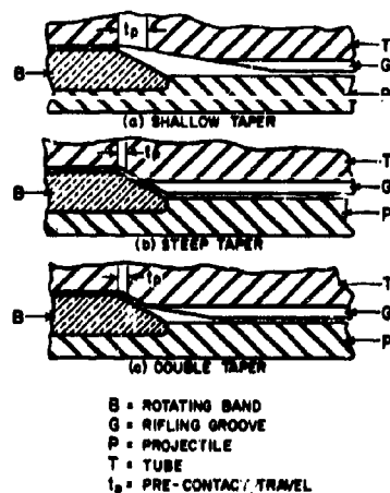
FIGURE 19. Forcing Cone Study.
