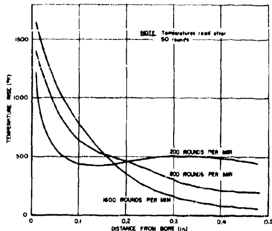
FIGURE 8. Temperature Distribution Across Tube Wall.
