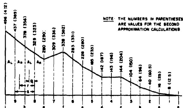
FIGURE 13. M/I Diagram of Gun Tube.
