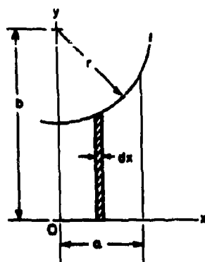
FIGURE 21. Nozzle Entrance Geometry.
