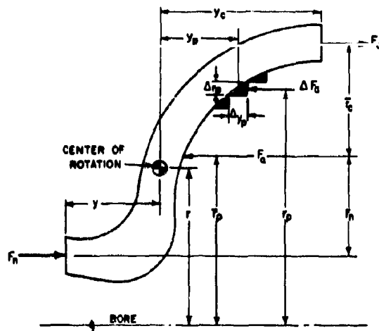
FIGURE 47. Toroidal External Loads.
