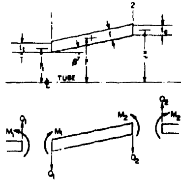
FIGURE 44. Conical Section Loading.
