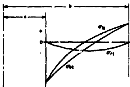
FIGURE 34. Thermal Stress Distribution Across Tube Wall.
