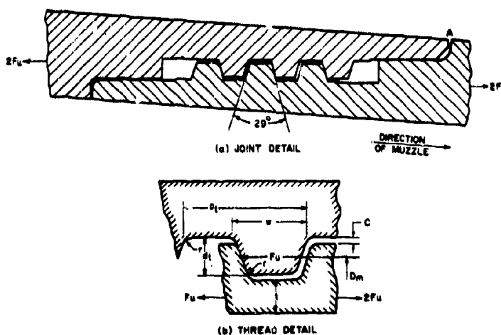
FIGURE 52. Threaded Joint.
