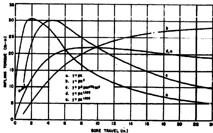
FIGURE 32. Rifling Torque Curves for Caliber .30 Barrel.
