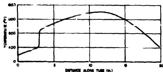
FIGURE 9. Temperature Along Outer Surface of Caliber .30 Tube.
