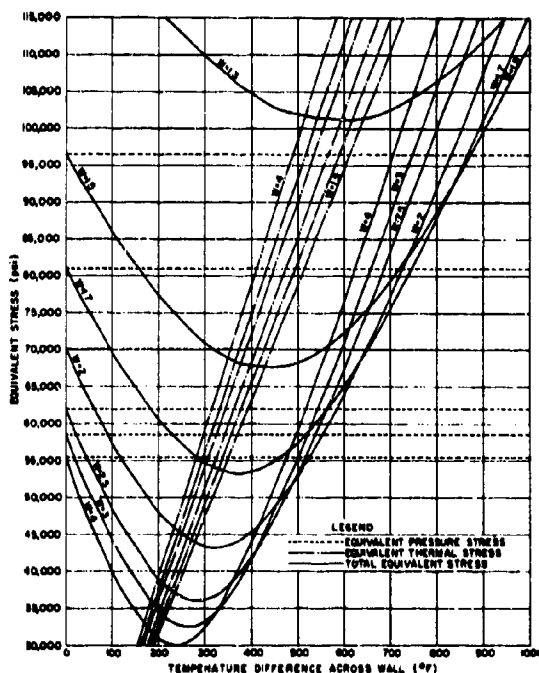
FIGURE 37. Equivalent Stress as a Function of Wall Thickness Ratio and Temperature Distance for an Internal Pressure of 50,000 psi.
