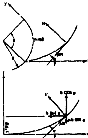
FIGURE 28. Rifling Force Diagram.
