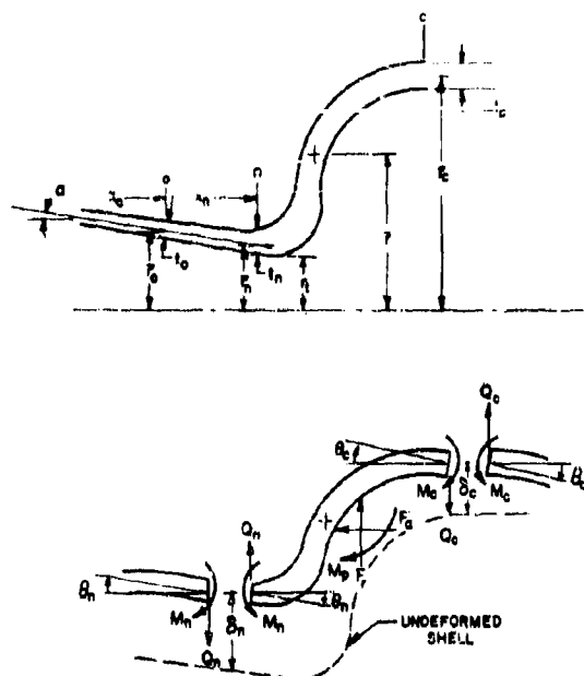
FIGURE 45. Toroidal Section Loading.
