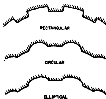
FIGURE 14. Types of Rifling Contour.
