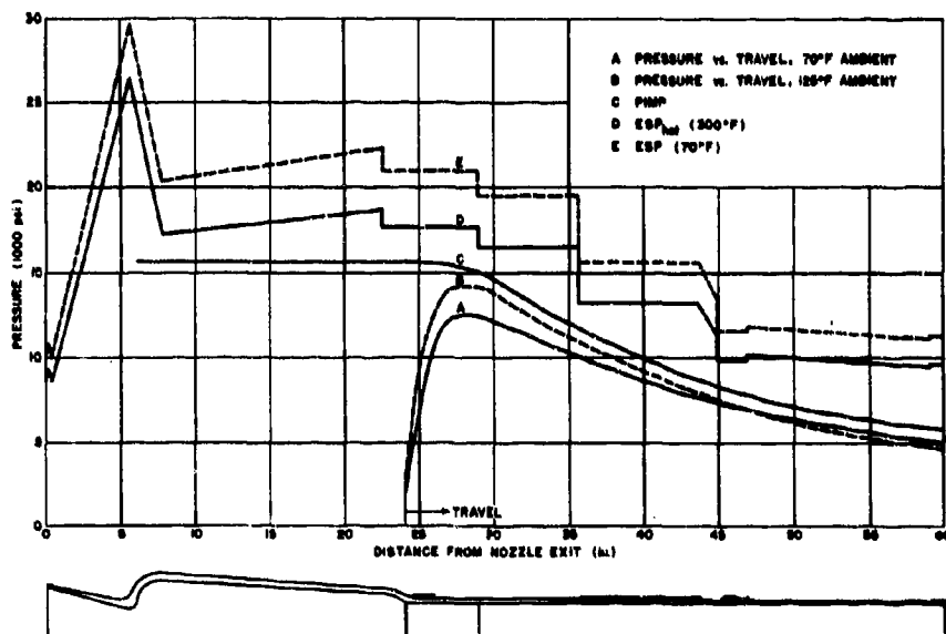
FIGURE 42. Typical Recoilless Gun Pressure Design Curves. (For hypothetical gun only)
