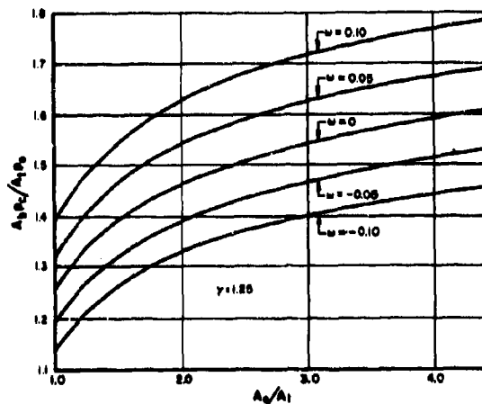
FIGURE 23. Lines of Constant Dimensionless Recoil.
