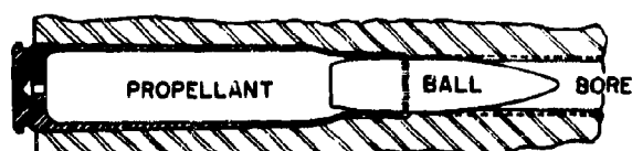
(b) SMALL ARMS CHAMBER CONTAINING FIXED ROUND
