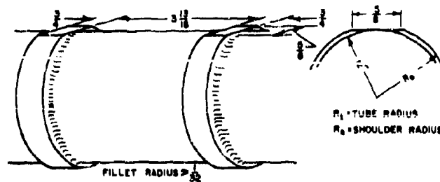
FIGURE 54. Gunner's Quadrant Flats.
