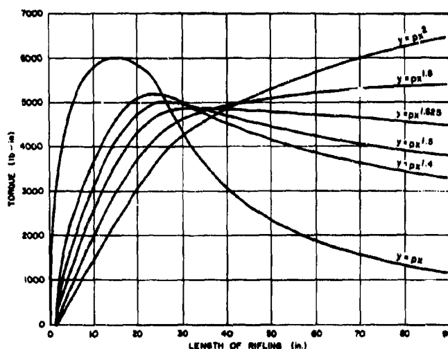
FIGURE 29. Torque Curves for 37 mm Gun.
