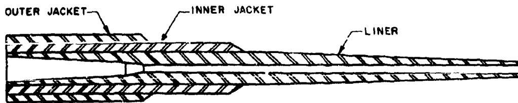
FIGURE 3. Jacketed Tube.
