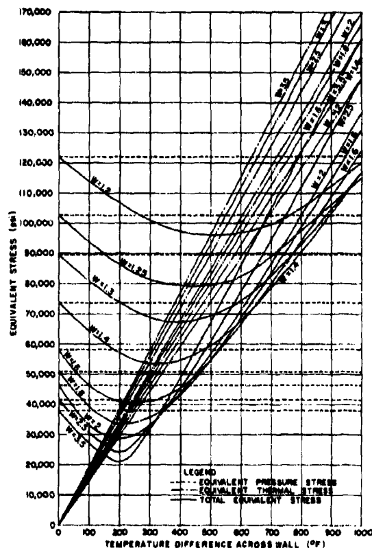
FIGURE 36. Equivalent Stress as a Function of Wall Thickness Ratio and Temperature Distance for an Internal Pressure of 20,000 psi.
