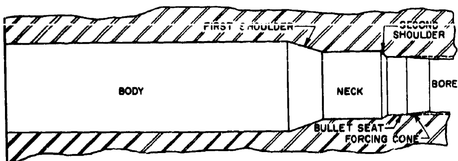
(a) CHAMBER SHOWING COMPONENTS
