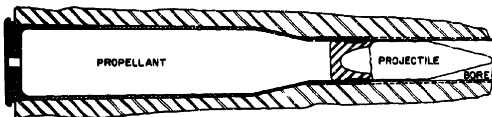
(c) ARTILLERY CHAMBER CONTAINING FIXED ROUND
