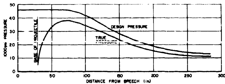
FIGURE 41. Design Pressure-Travel Curve.
