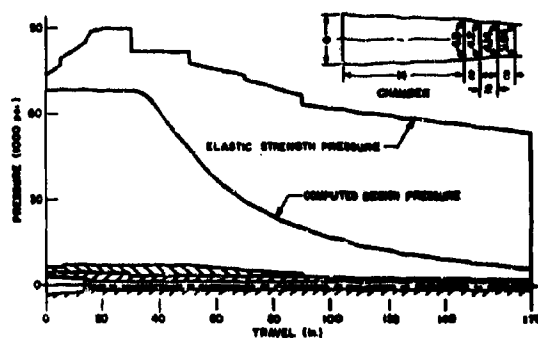
FIGURE 62. Design Data, Jacketed Artillery Tube.
