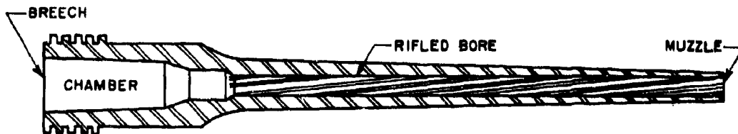
FIGURE 1. Typical Gun Tube Showing Regions.
