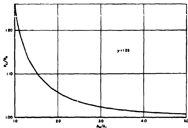
FIGURE 22. Pressure Ratio-Area Ratio Curve.
