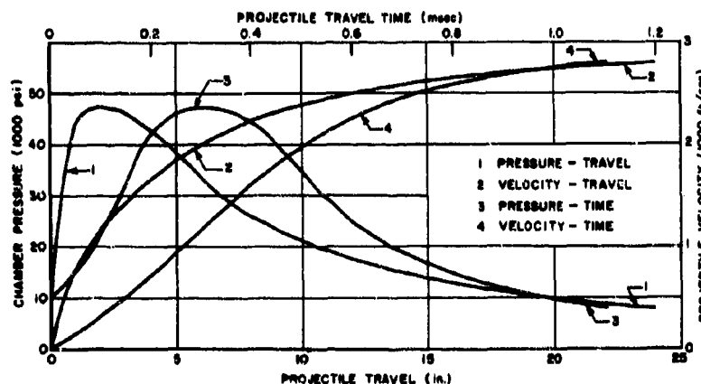
FIGURE 16. Interior Ballistics of Caliber .30 Gun.
