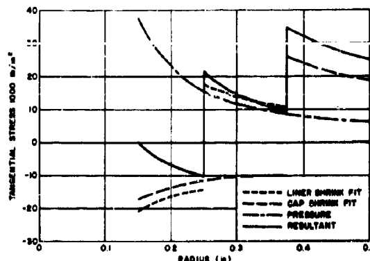
FIGURE 64. Tangential Stress of Shrink Fitted Tube.
