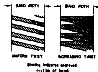
FIGURE 15. Progressive Engraving.
