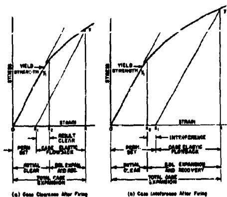
FIGURE 17. Case-Chamber Stress-Strain Curves.
