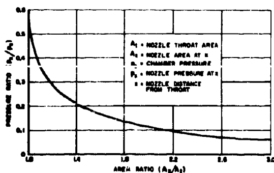
FIGURE 25. Nozzle Pressure-Area Ratio Curve, M10 Propellant.
