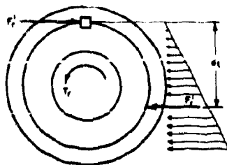
FIGURE 53. Rifling Torque Reactions.
