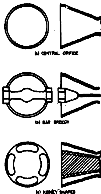
FIGURE 24. Nozzle Shapes-Schematic.
