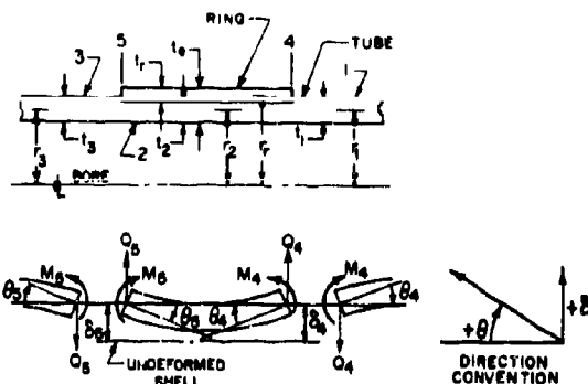
FIGURE 43. Gimbal Ring Loading.
