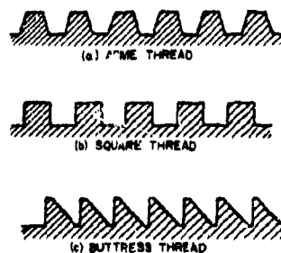
FIGURE 50. Thread Profile Types.
