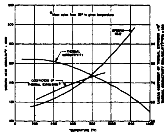
FIGURE 58. Physical Properties of Steel.
