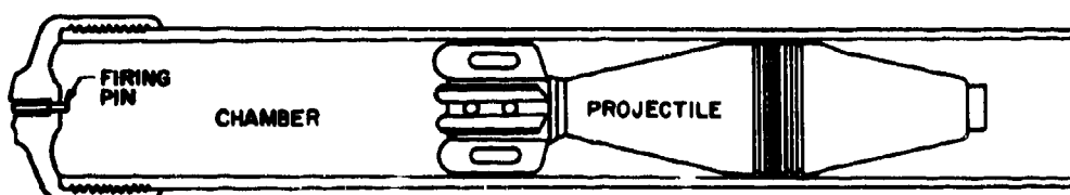
FIGURE 2. Chambers of Various Tube Types.
