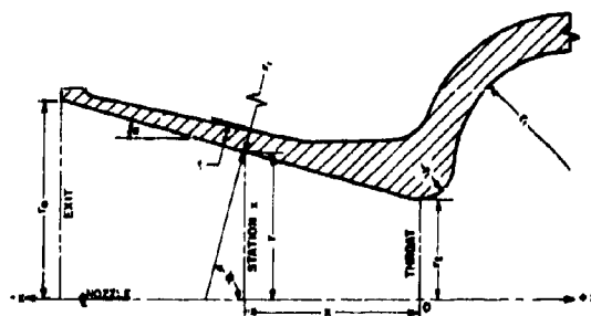
FIGURE 48. Nozzle With General Dimensions.
