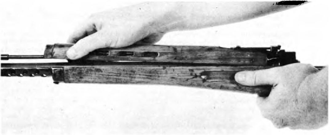
FIGURE 70. REMOVING THE HANDGUARD.
