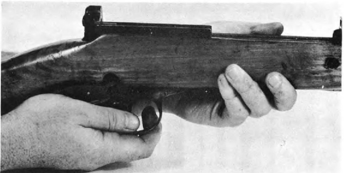
FIGURE 67. REMOVING TRIGGER MECHANISM (STEP 2).
