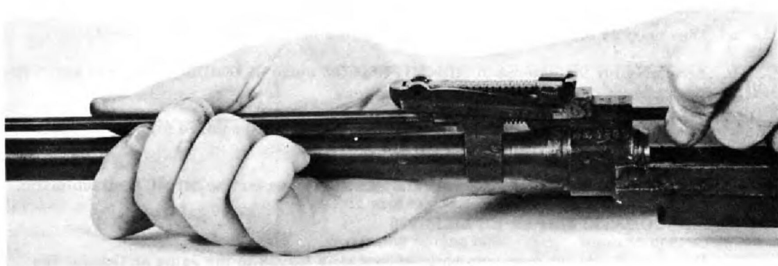
FIGURE 73. REMOVING THE OPERATING ROD
