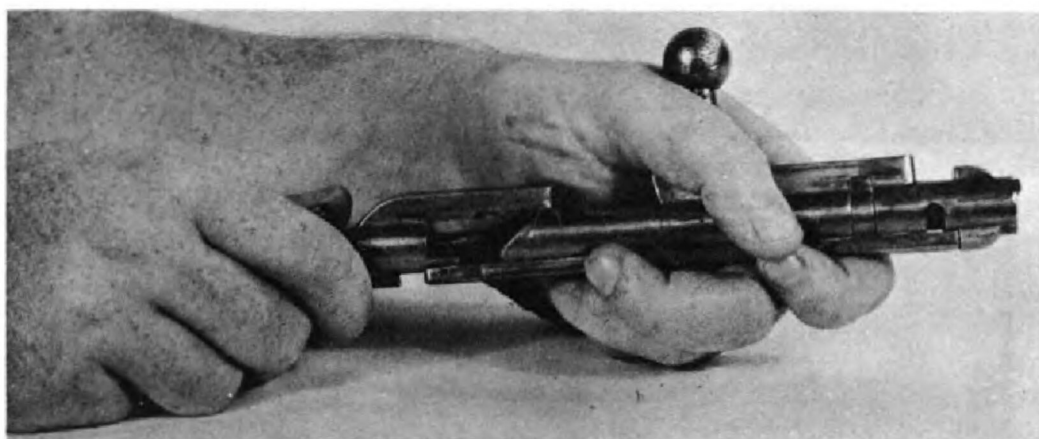
FIGURE 45. REMOVING THE BOLT.
