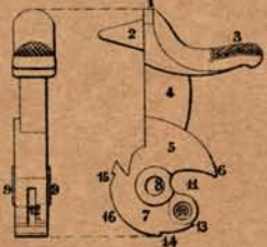
Fig 18. Grand ressort
