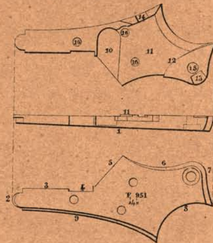
Fig 6. Plaque de recouvrement.
