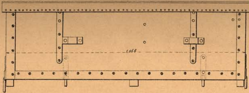
Fig. 1. Elevation.
