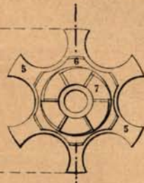
Fig.11 Support de barillet.
