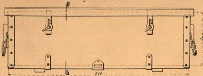
Fig. 7. Elevation.
